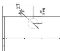
CROSS SECTION
